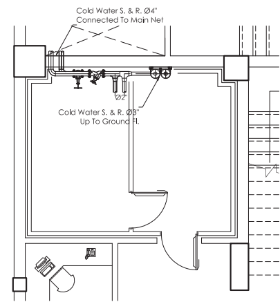
Basement Part Plan Scale 1 : 50
