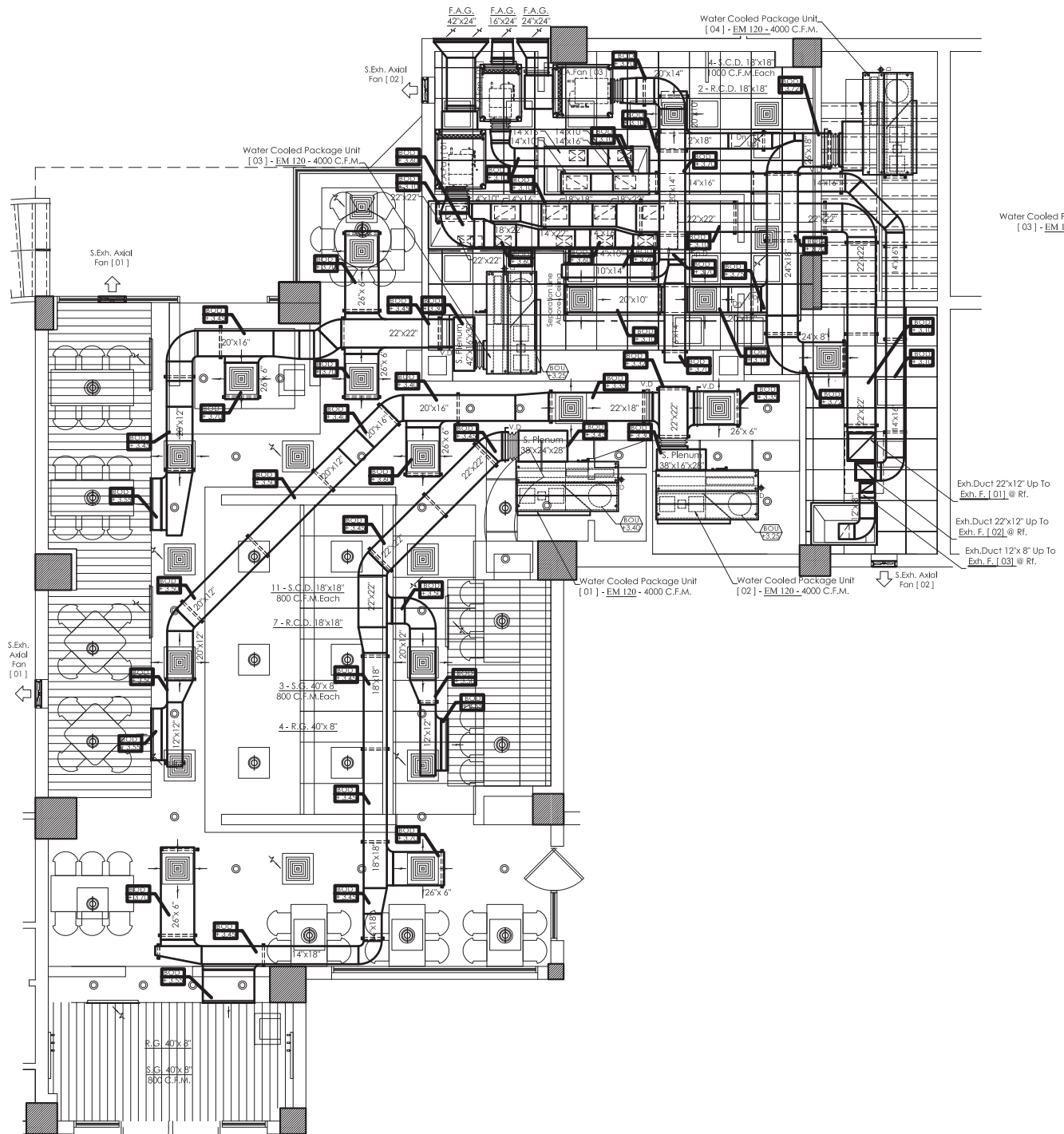
Restaurant Plan Scale 1 : 50
