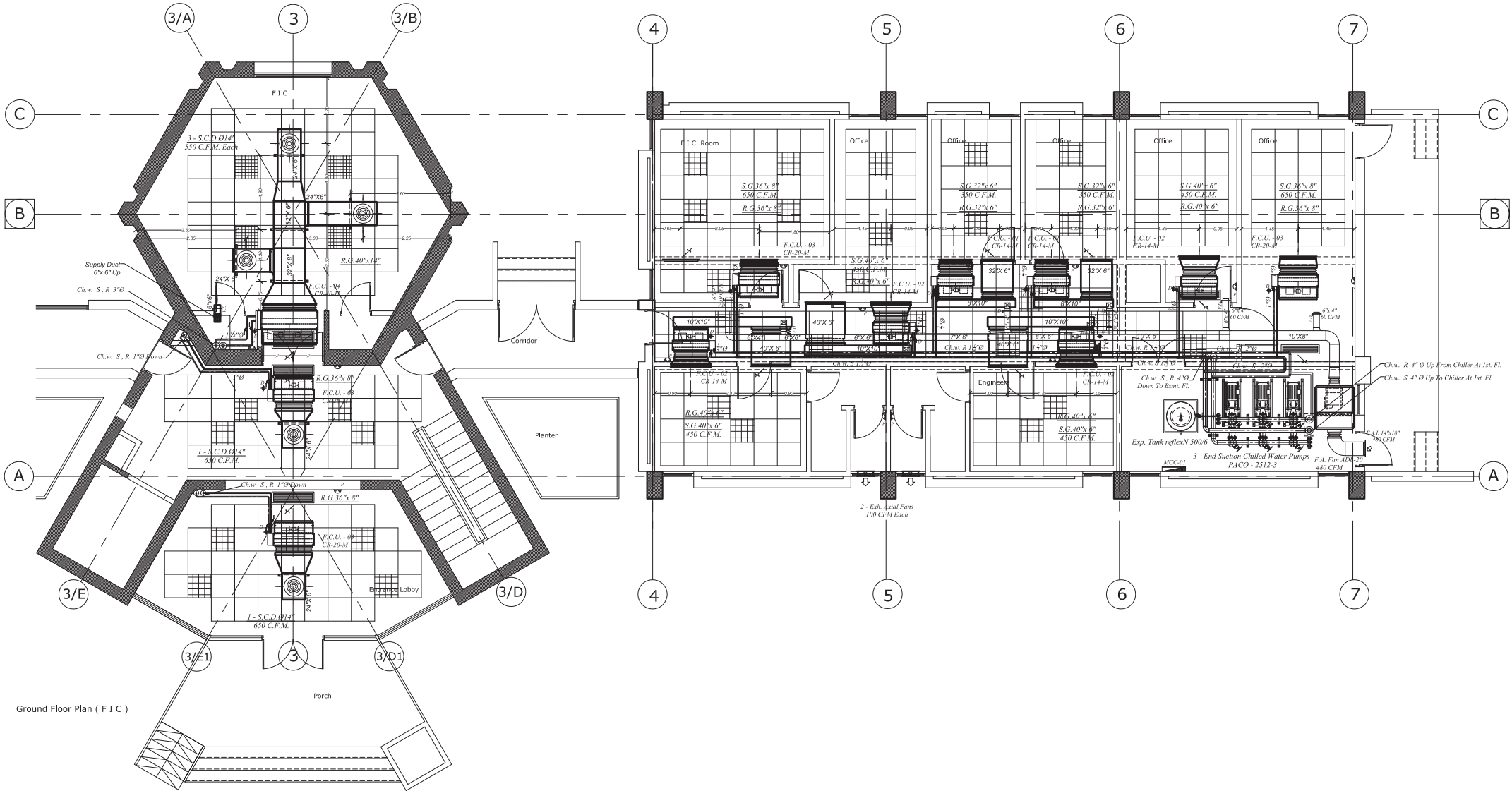
Control Tower Luxor Airport Ground Floor
