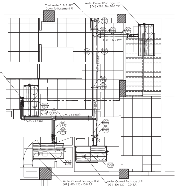
Restaurant Part Plan Scale 1 : 50
